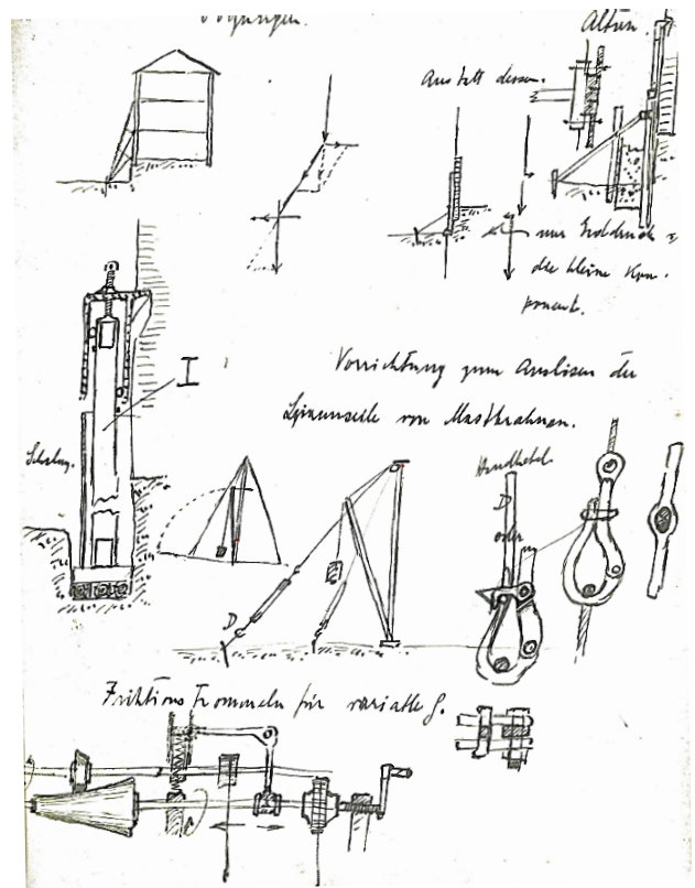
Figure 6. Installations and equipment for clearing work (Note II-1).
