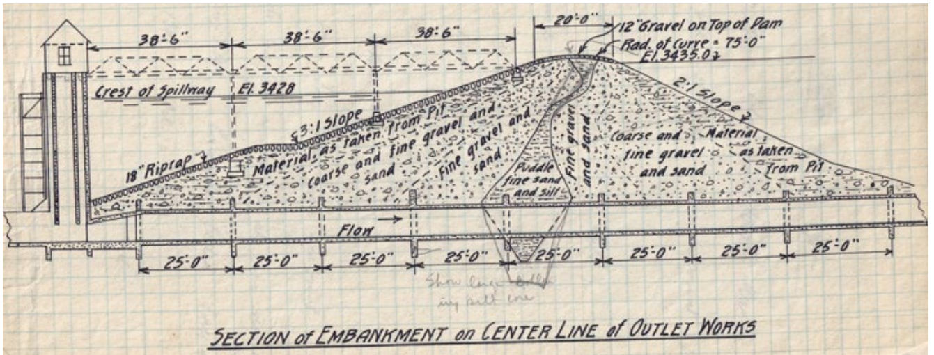
Figure 5. Cross-section, Yakima Project (Note 17). Dimensions in ft and inches.
